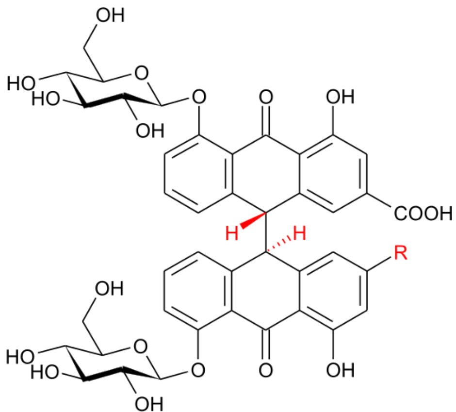
Sennosid A: R = \text{COOH} Sennosid C: R = \text{CH}_2\text{OH}
