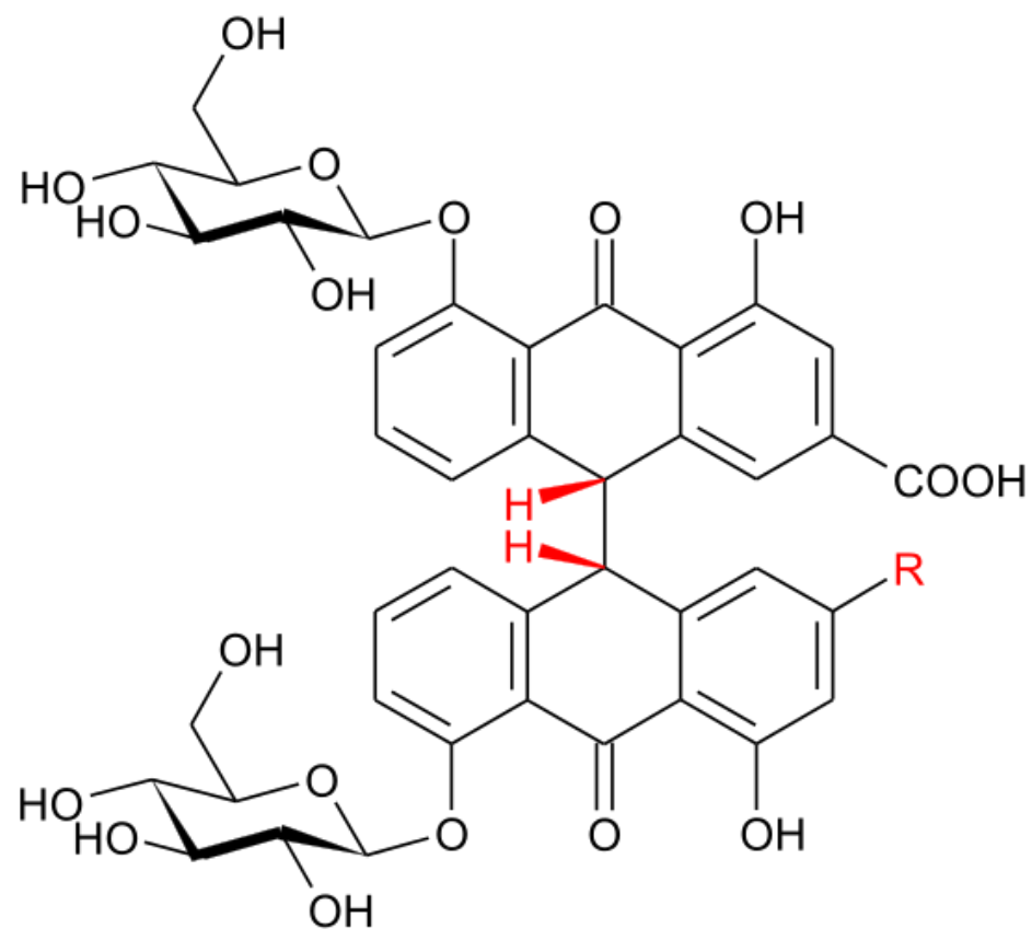
Sennosid B: R = \text{COOH} Sennosid D: R = \text{CH}_2\text{OH}
