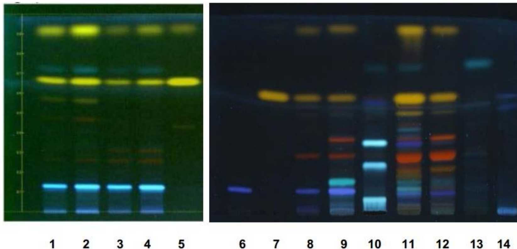
Typical HPTLC Chromatograms
